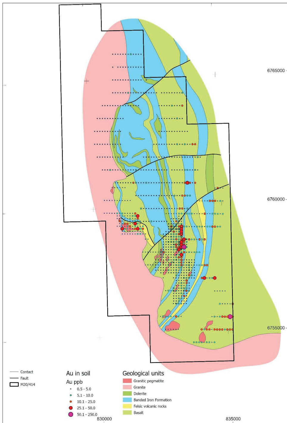
Figure 1: Geochem gold-in-soil anomalies from the 2023 Phase 1 and 2 programs.
