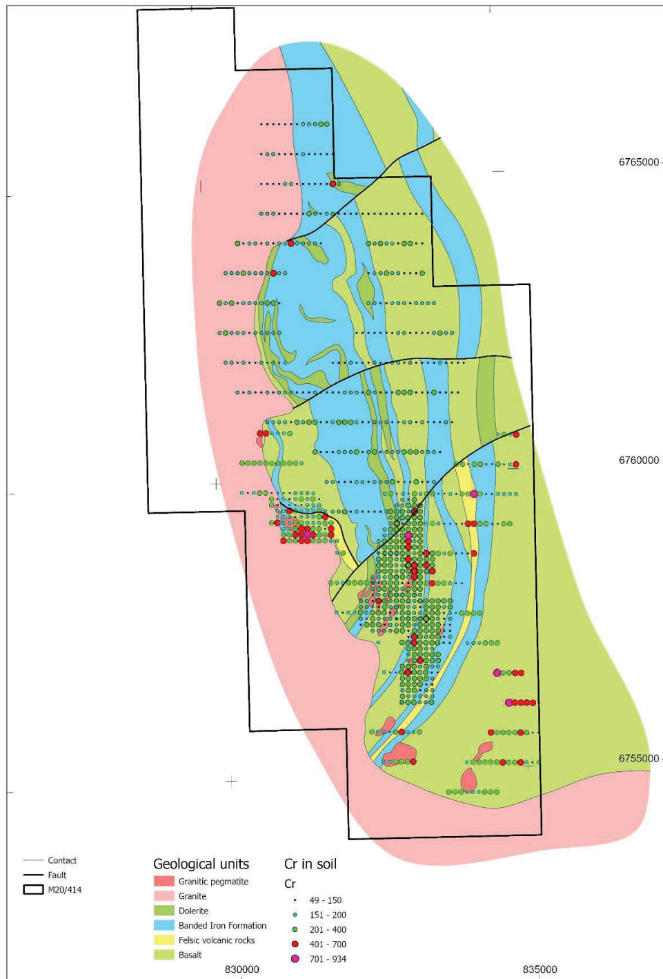
Figure 3: Geochem chromium-in-soil anomalies from the 2023 Phase 1 and 2 programs.
