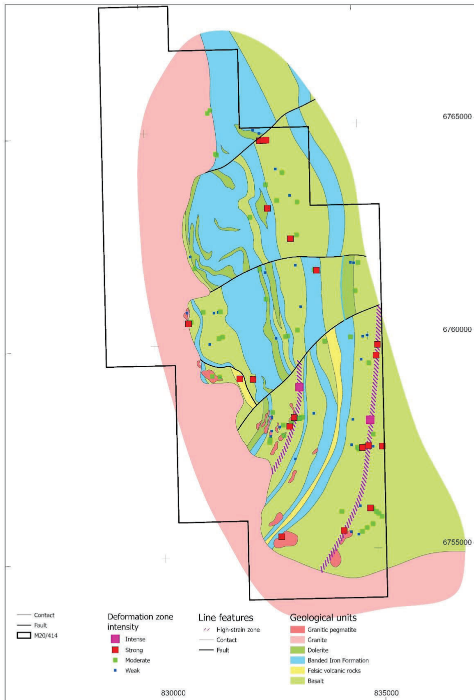
Figure 2: Mount Ida Structure Lines.
