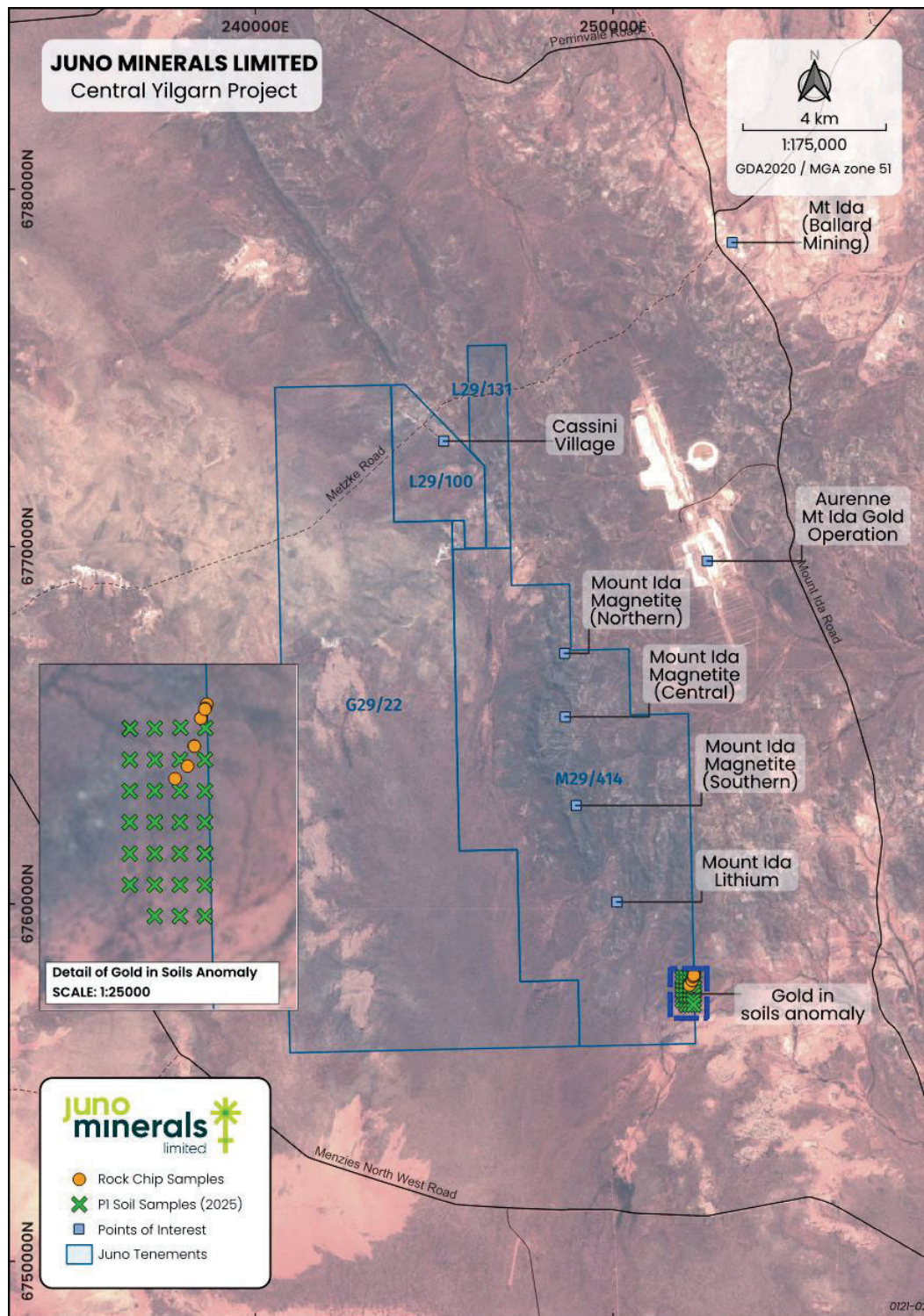
Figure 4: Southern gold-in-soils anomaly.
