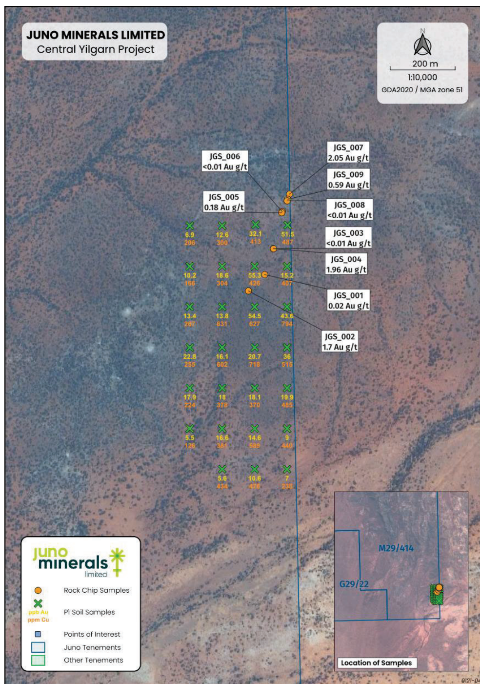
Figure 5: Rock chip samples and gold-in-soils anomaly extension
